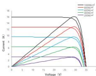
I-V/P-V Curve at Different Irradiation SSA-48HDB-445N
